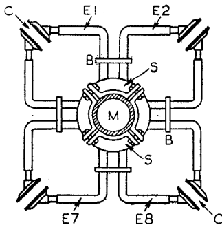
Aerial for circular radiation.
