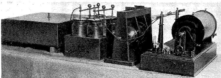
It was with gear like this that the outstanding achievements of the early days of wireless telegraphy were accomplished "in spite of principles and theory". This Marconi transmitter, exhibited at the I.E.E. Wireless Section Commemoration Meeting, comprises (right to left) induction coil, spark gap, Leyden jar battery and "jigger" (aerial coupling transformer)
