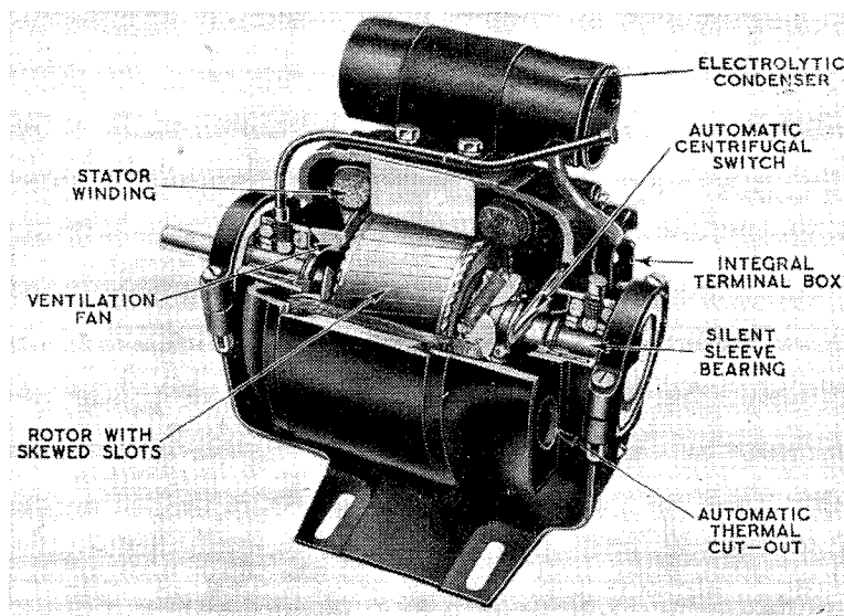
Cut-away view of a typical small induction motor, made by G.E.C., showing construction and salient features.
