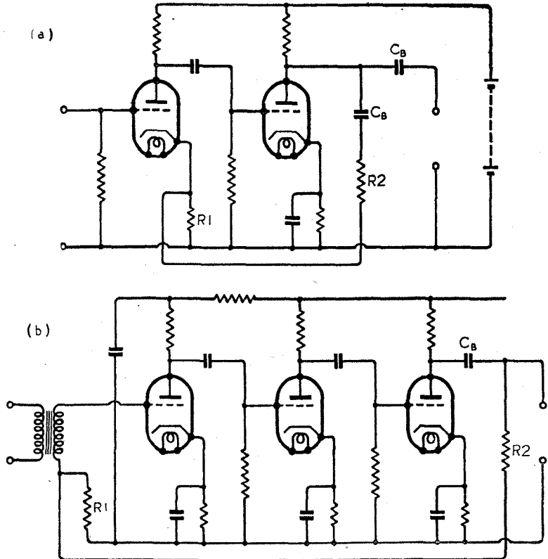
Fig. 5. (a) Two-stage feedback amplifier. (b) Three-stage feedback amplifier. The feedback depends on R_1 and R_2 .
